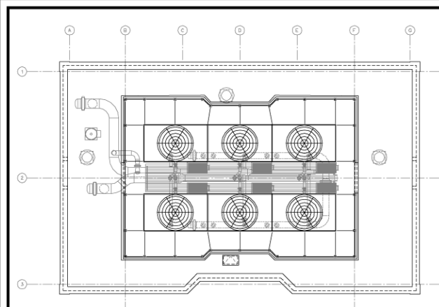
SCREEN WALL PLAN
