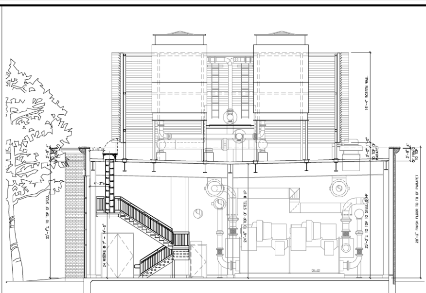
BUILDING SECTION
