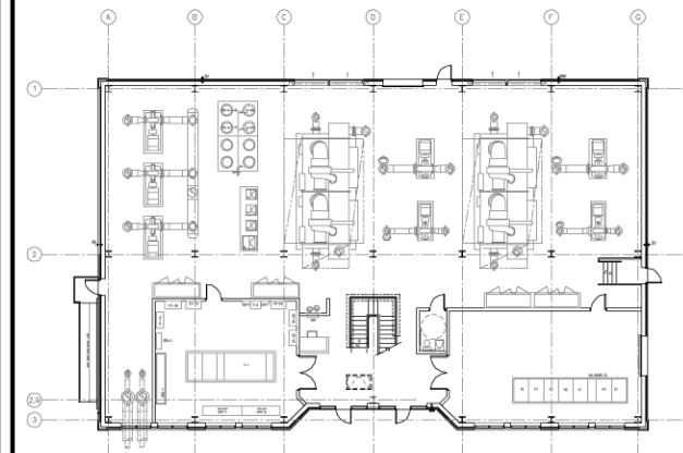
OPERATING FLOOR
