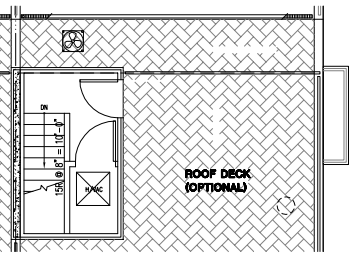
PENTHOUSE (PARTIAL) *FINAL LAYOUT SUBJECT TO CHANGE*
