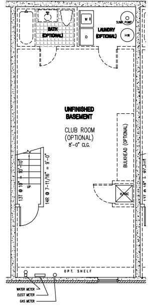
BASEMENT *FINAL LAYOUT SUBJECT TO CHANGE*
